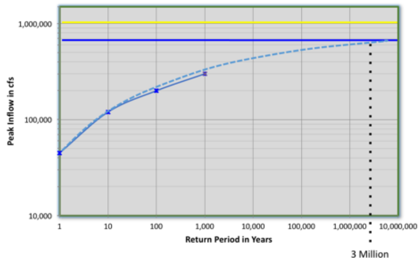
Figure 3, Historic Peak Flows Extrapolated showing PMF limit
